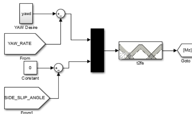
Fig11. Fuzzy controller schematic in our MATLAB Simulink environment
