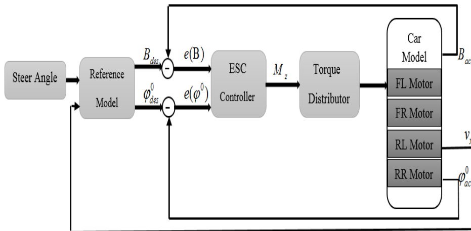
Fig9.. Overall structure of our ESC control system
